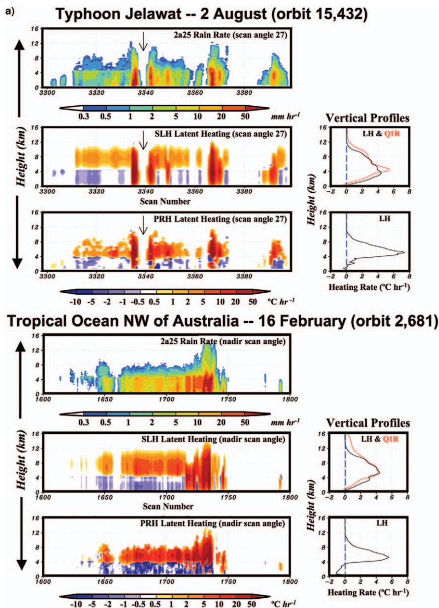
FIG. 5a. (top five) LH analysis for tropical Pacific Typhoon Jelawat in developing stage (2 Aug 2000). Arrows indicate location of eye and (bottom five) identical analysis for tropical, oceanic MCS over northwest Australia (16 Feb 1998). (left) For each set of diagrams height-scan cross sections of PR-based rain-rate profiles ( \text{mm h}^{-1} ), along with SLH- and PRH-generated LH profiles ( ^\circ\text{C h}^{-1} ), are shown respectively. [TRMM PR rain-rate algorithm is described by Iguchi et al. (2000) and Meneghini et al. (2000).] (right) area mean vertical profiles of both SLH-generated Q_i - Q_R (red) and LH (black) and PRH-generated LH (black) in ^\circ\text{C h}^{-1} , respectively.
